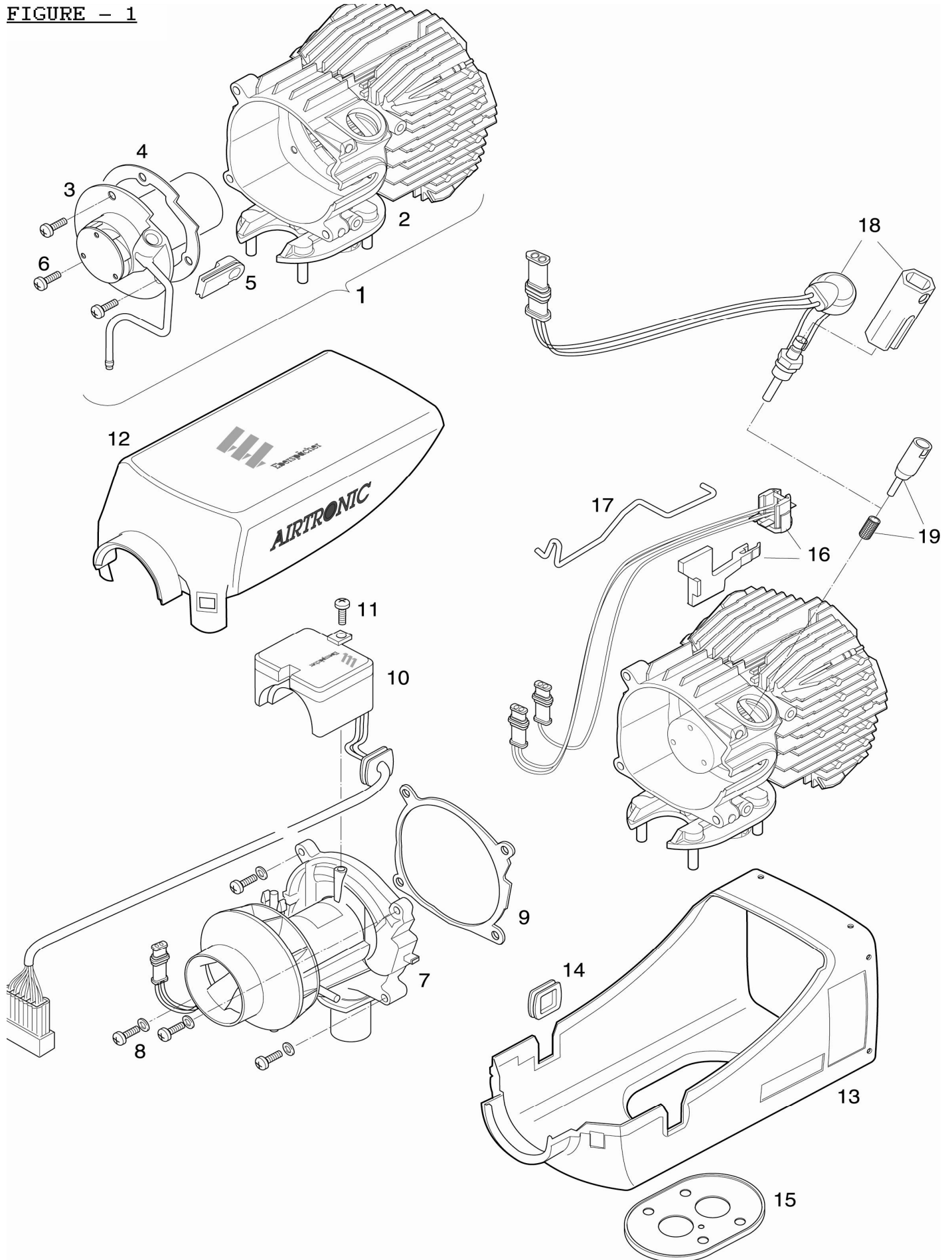
YARDIMCI ISITICI DETAYLARI AUXILIARY HEATER DETAILS
